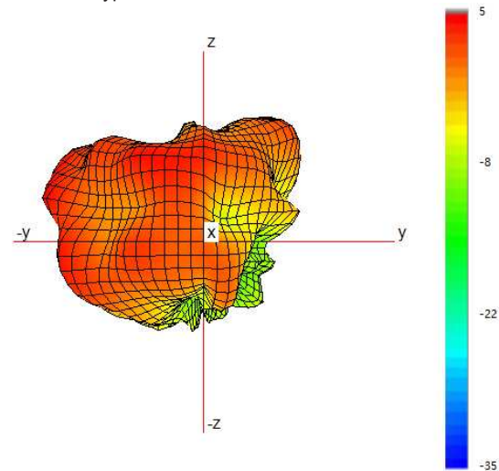
Typical 3D Pattern- WiFi - 3 - 6500 MHz
