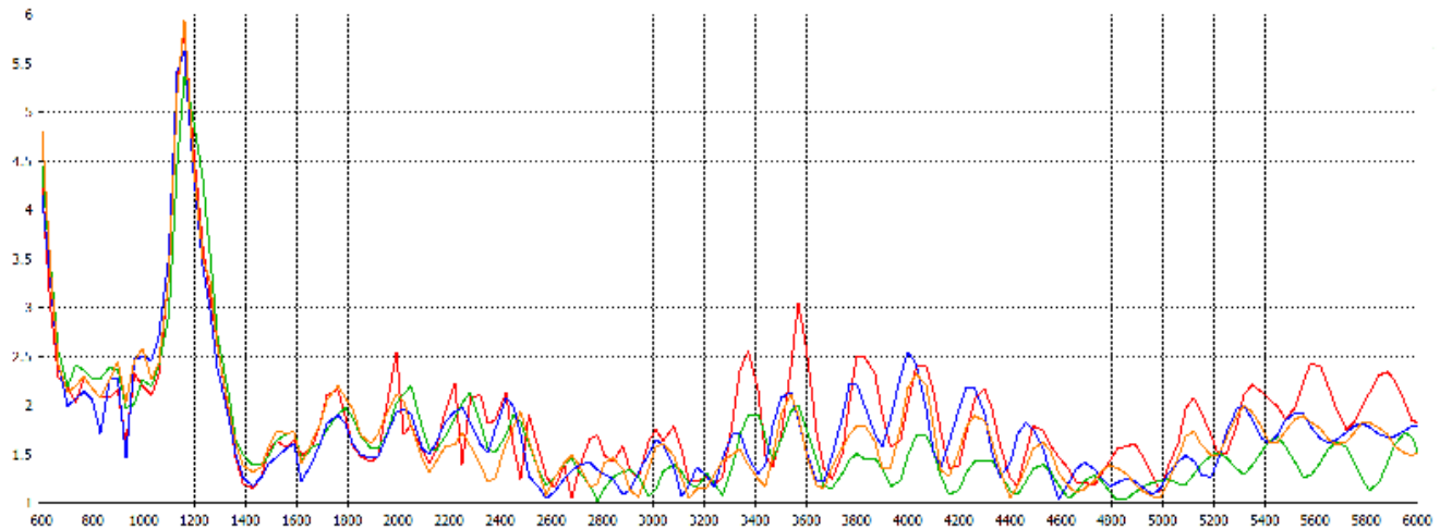
Typical VSWR*
