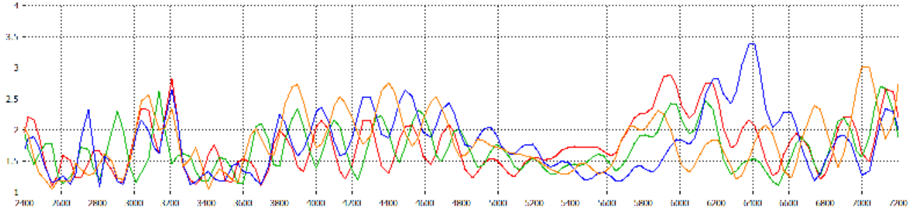
Typical VSWR*
