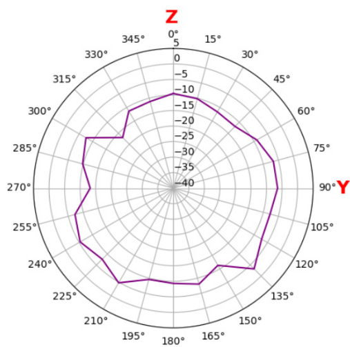
Aux GPS yz plane
