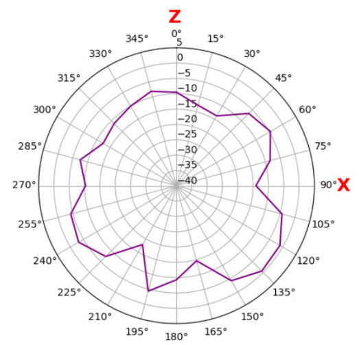
Aux GPS xz plane
