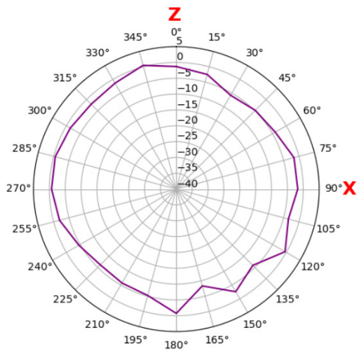
Aux B13 750 MHz xz plane
