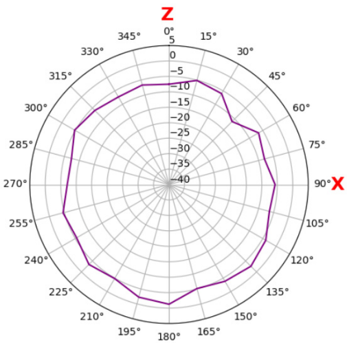
Aux B7 2650 MHz xy plane
