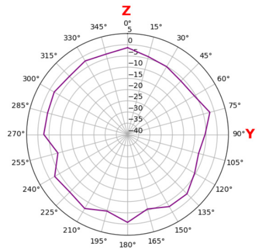
Aux B13 750 MHz yz plane
