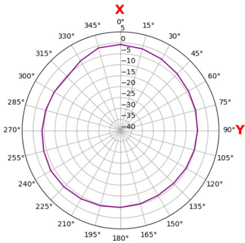
Main B7 2550 MHz xz plane
