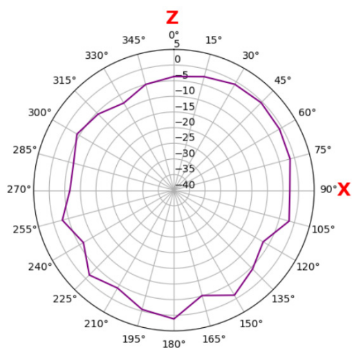
Main B2 1860 MHz yz plane
