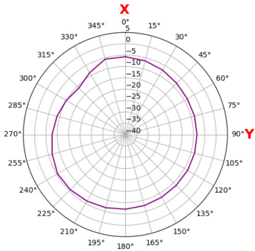
Aux B2 1950 MHz xz plane
