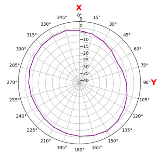
Aux B13 750 MHz xy plane
