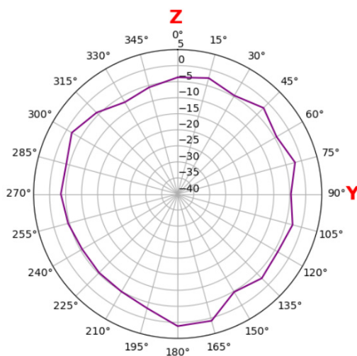
Main B7 2550 MHz xy plane
