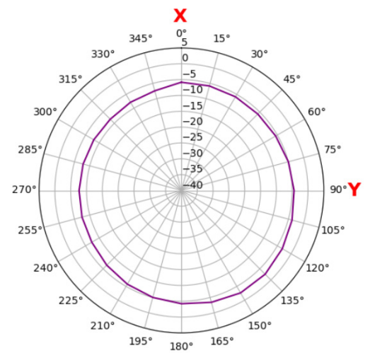
Main B13 780 MHz xz plane
