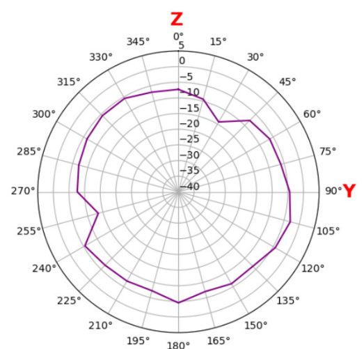
Aux B2 1950 MHz xy plane
