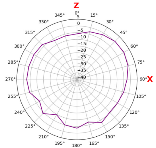
Aux B2 1950 MHz yz plane
