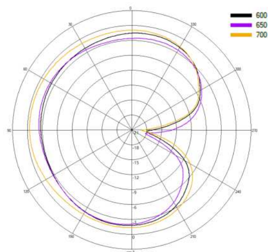
Typical H Plane- Cell A - Patterns- 600-700MHz
