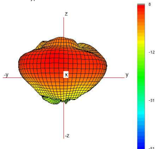
Typical 3D Pattern- WiFi - 4 - 2450 MHz
