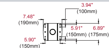
CEILING PLATE DETAIL
