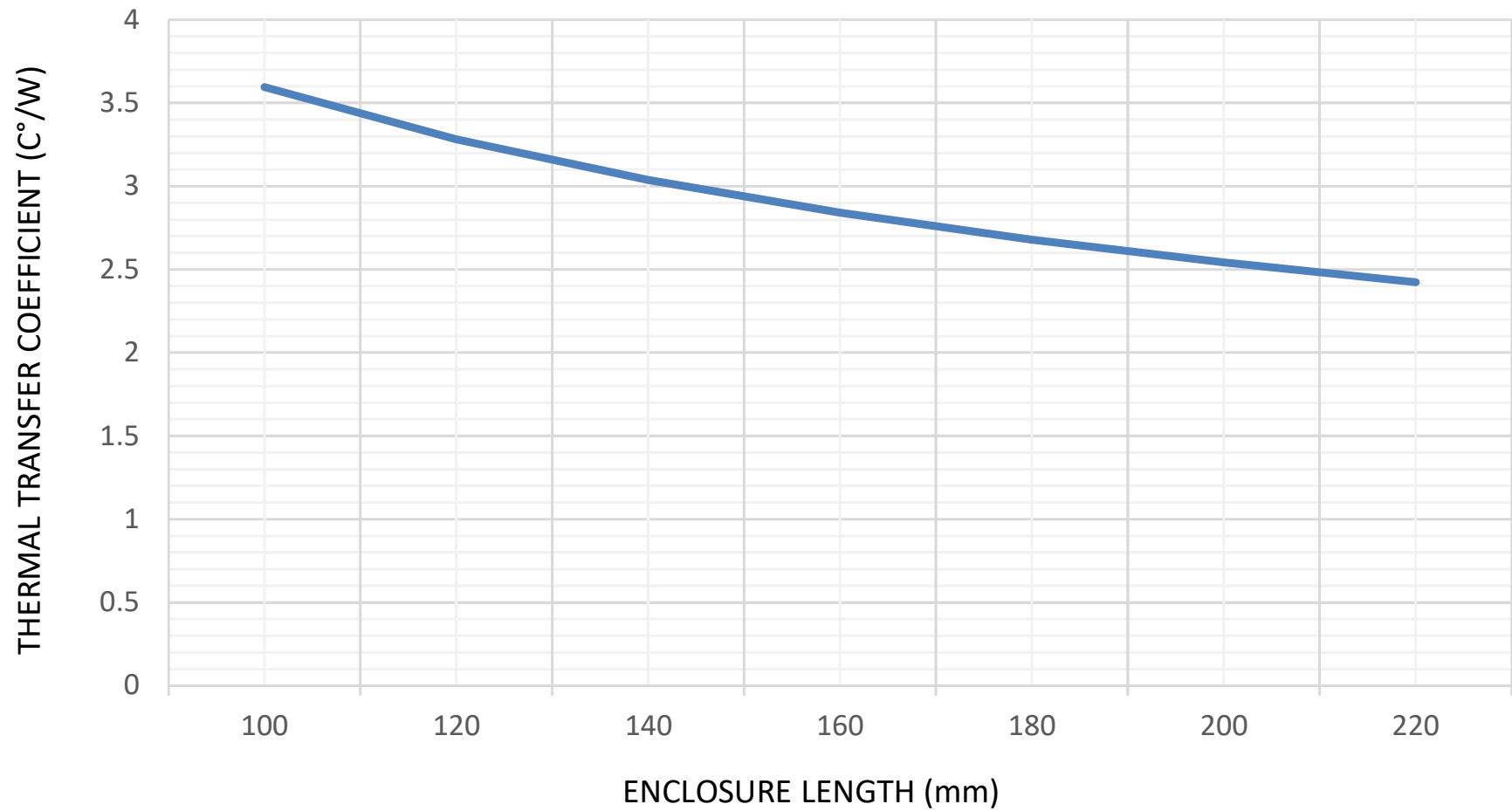
1455KHD Rth (C°/W) VS. ENCLOSURE LENGTH
