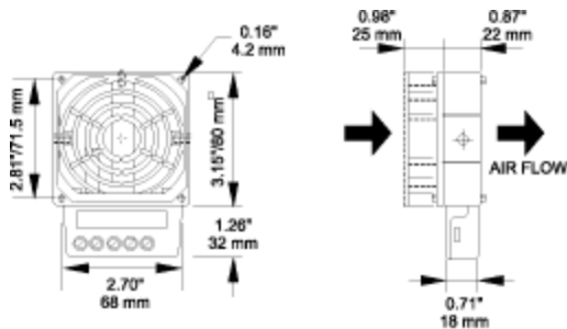
100 W, 150 W Heaters
