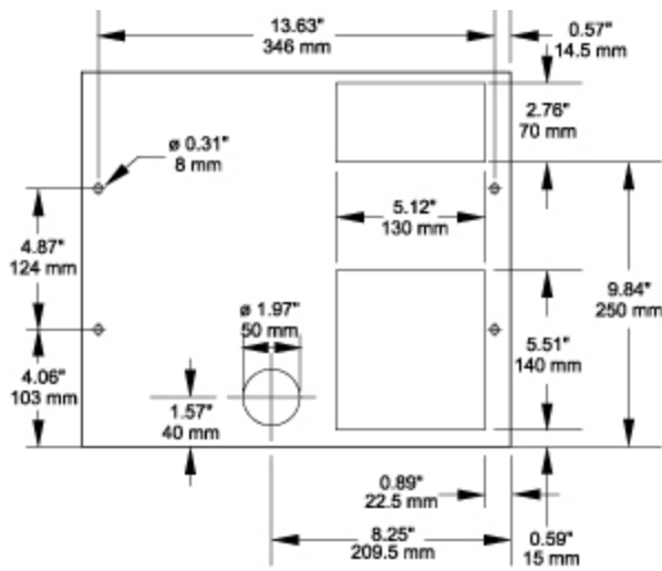
Drilling Template
