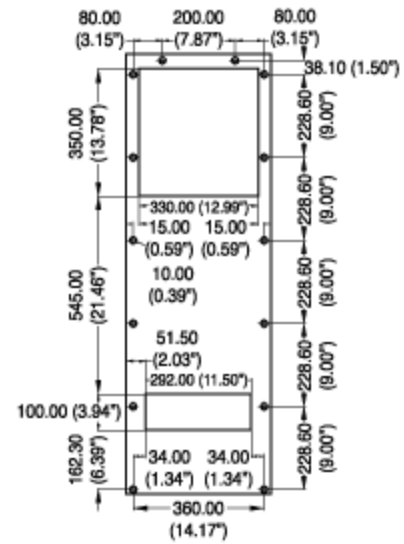
Drilling Template
