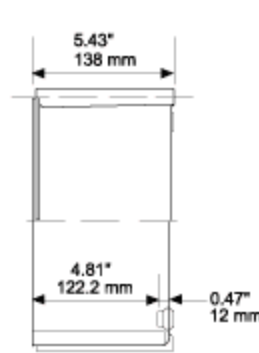
Base Front View PB271818, PB272718, PB362718
